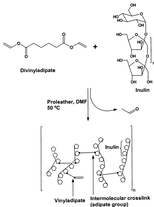
Scheme 1. Schematic Representation of Enzyme-Polytransesterification of Inulin with DVA
